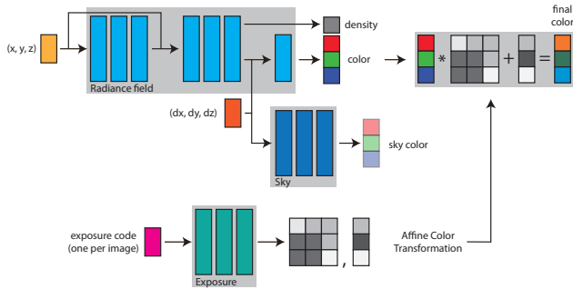
Figure 9. Network architecture
